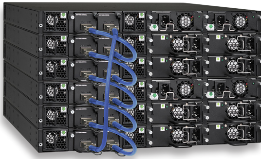
Figure 1: Up to 12 Ruckus ICX 7450 switches can be stacked together using two full-duplex QSFPP+ 40 Gbps ports that provide a fully redundant backplane with 960 Gbps of stacking bandwidth.
